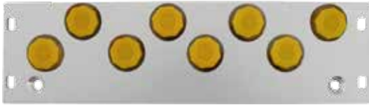
REF. 9D.FO159-8ST MOD. SMT 3U 7TE 8ST/FC + ADAPT + PIGT+NUMER
