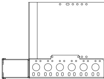
REF. 9D.FO160.4Un SubRack 19"4u 84TE S/Slot Negro
