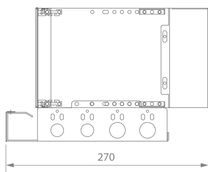
REF. 9D.FO160.4Up SubRack 19"4u 84TE S/Slot Plata
