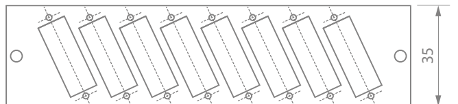
FRONT 8DSC/LC
