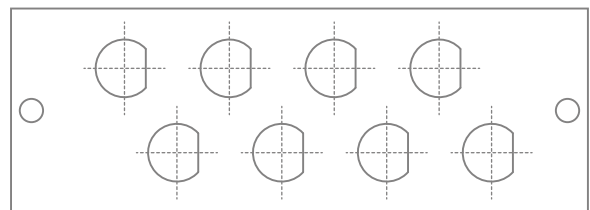
FRONT 8ST/FC
