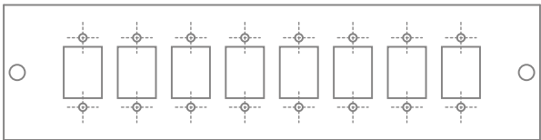
FRONT 8SC/E2000
