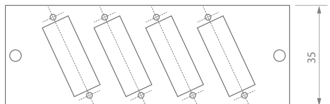
FRONT 8SC/E2000
