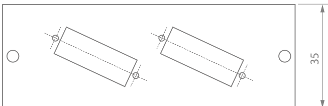
FRONT 4SC/E2000
