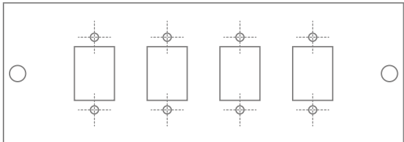
FRONT 4SC/E2000
