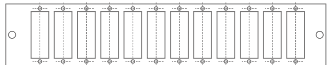
FRONT 12DSC/LC
