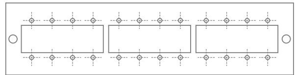
FRONT 12SC/E2000
